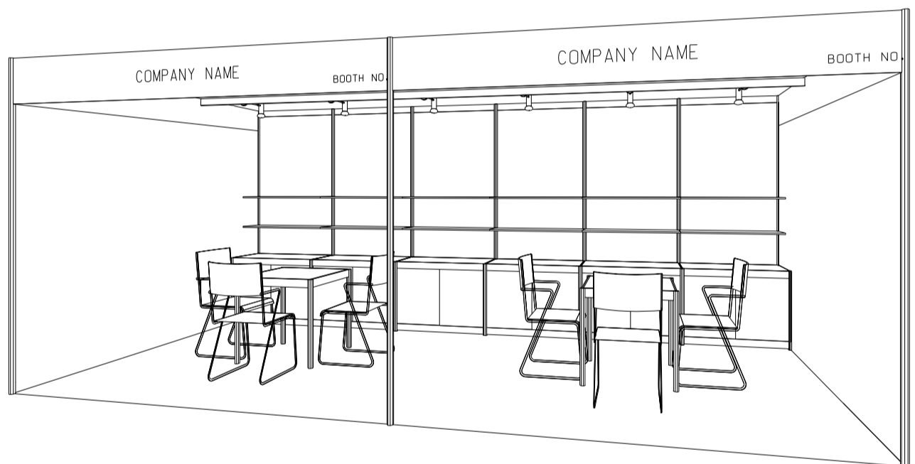
PERSPECTIVE 6M(W) X 3M(D) X 2.5M(H) Peninsula Booth A
