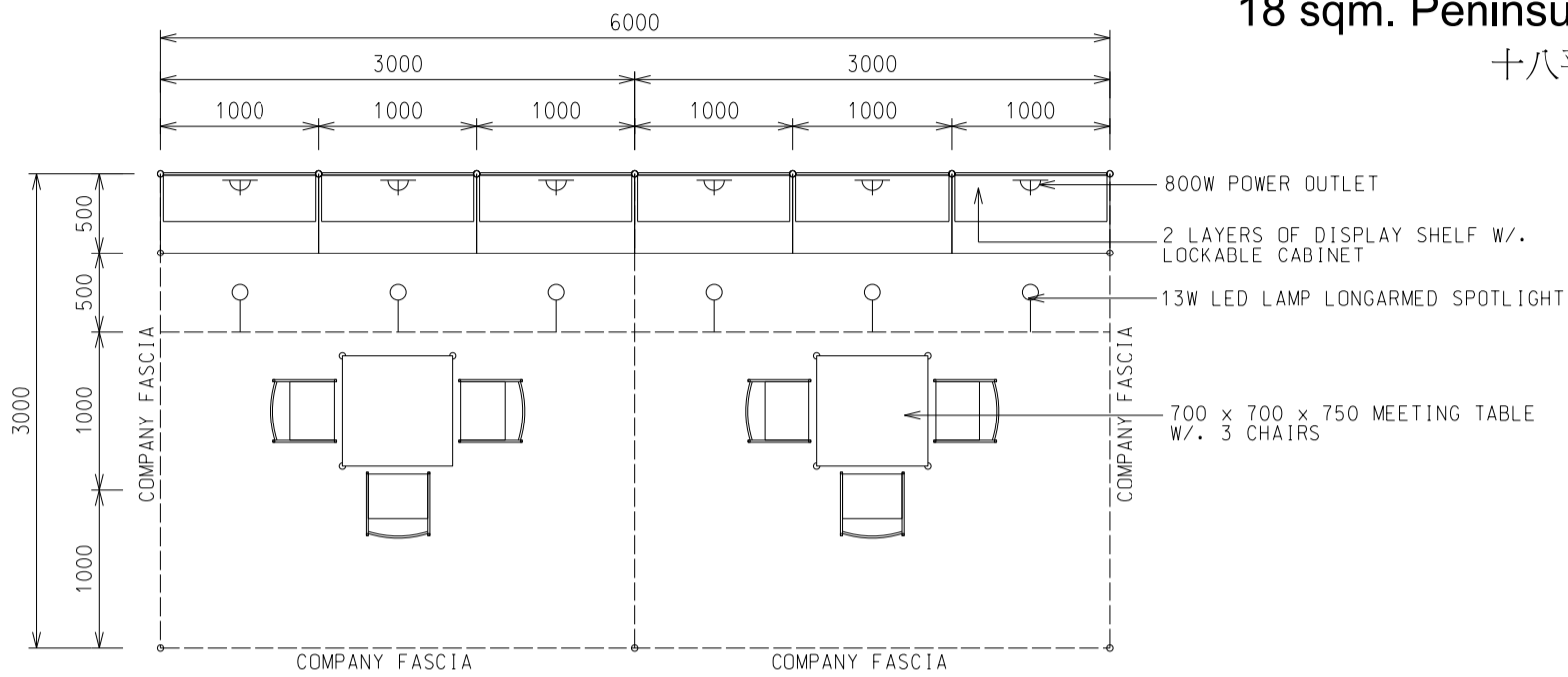
PLAN 6M(W) X 3M(D) X 2.5M(H) Peninsula Booth A
