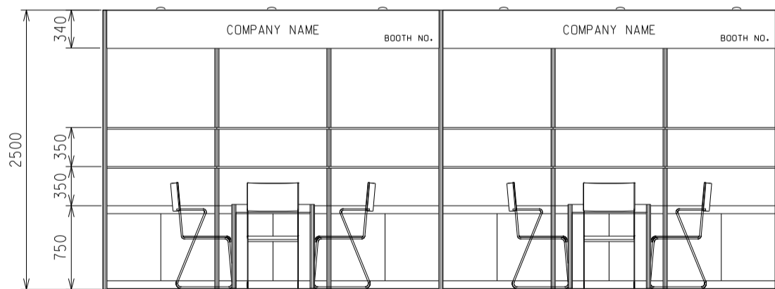
ELEVATION 6M(W) X 3M(D) X 2.5M(H) Peninsula Booth A
